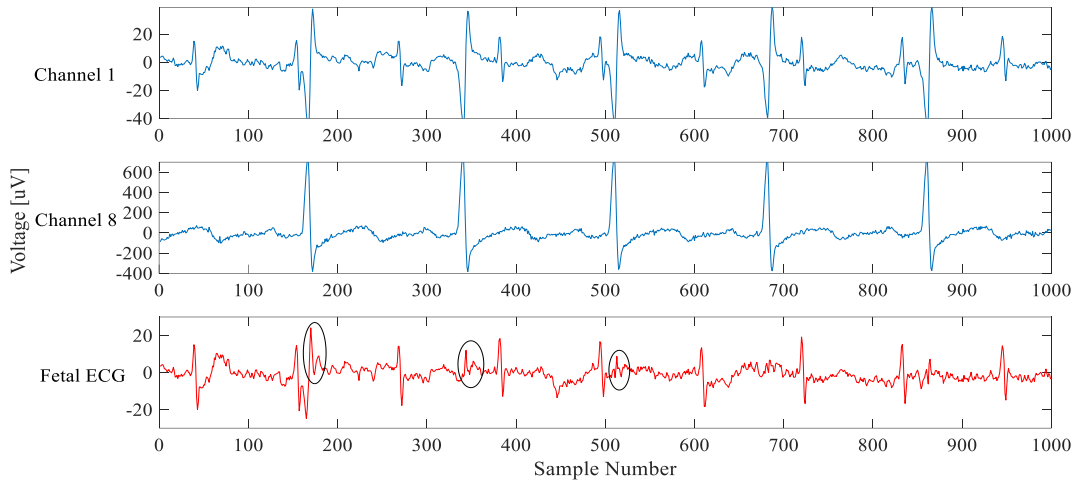
Figure 4. Fetal ECG signal obtained by least mean squares (LMS) method.
