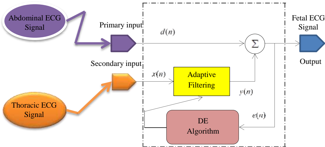
Figure 2. Block diagram for combining and applying DE algorithm with adaptive filtering.
